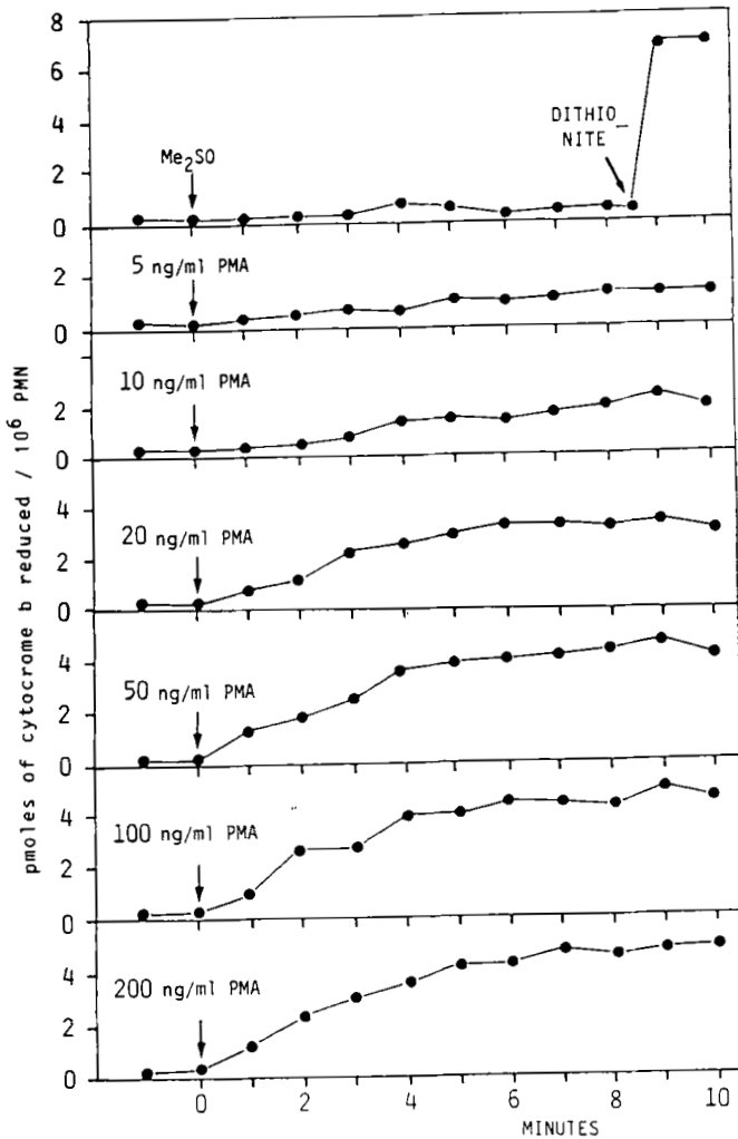
FIGURE 5 Kinetics of endogenous reduction of cytochrome b_{-245} by PMA-activated neutrophils. Two cuvettes were filled with 2 ml of neutrophil suspension ( 4 \times 10^7 cells/ml) in incubation buffer supplemented with 200 U/ml catalase and placed in the compartment for turbid samples of a double beam spectrophotometer thermostated at 37°C and equipped with magnetic stirring. In this experiment the cells were not pre-labeled with ^{32}\text{P} i. To the sample cuvette 0.4 mg of glucose oxidase were added and the cuvette was immediately closed with a plug bearing two needles, one for a continuous inlet of oxygen-free nitrogen and the other for the outlet of the gas and the addition of the stimulant. The reference cuvette was not closed. After 10 min of equilibration, the indicated doses of PMA were added to the sample cuvette and spectra of reduced-oxidized cytochrome b were recorded at time intervals. Full reduction was achieved by addition of 20 \mu\text{l} of a fresh saturated solution of sodium dithionite.
